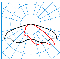
LIQ 70N-AB7L-LRA/75/82/91-727 10G1 ETDD(CLO end value) TX277813
