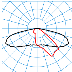
LIQ 50N-AB2L-LR/220/260/320-740 4G1 ET (CLO initial value) TX278137
