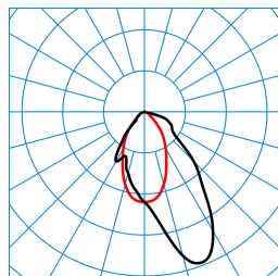
CreavoAct M59-TS LWW-03 53-8 ETDD8 01 (ACTDSU) TX195478 DIN 5040: A50 UTE: 1,00 C CEN Flux Code: 70 92 99 100 100 ■ C0 - C180 ■ C90 - C270
