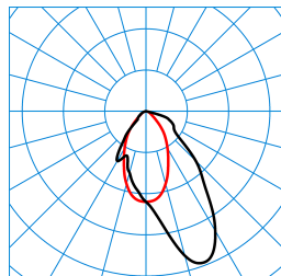
CreavoAct M59-TS LWW-03 53-8 ETDD8 01 (ACTDCW) TX195477 DIN 5040: A50 UTE: 1,00 C CEN Flux Code: 70 92 99 100 100 ■ C0 - C180 ■ C90 - C270
