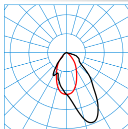
CreavoAct M59-TS LWW-03 53-8 ETDD8 01 (ACTDWW) TX195479 DIN 5040: A50 UTE: 1,00 C CEN Flux Code: 70 92 99 100 100 ■ C0 - C180 ■ C90 - C270
