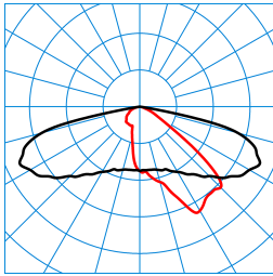
LIQ 50N-AB2L-LRA/1200-722 2G1 ETDD (CLO end value) TX281114
