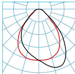
ArimoFit G2 Act D2 P-WW 42-8 ETDD8 01/01 (ACTDCW) TX377064 DIN 5040: A50 UTE: 1,00 C CEN Flux Code: 66 90 97 100 100
