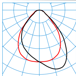
ArimoFit G2 Act D2 P-WW 42-8 ETDD8 01/01 (ACTDWW) TX377112 DIN 5040: A50 UTE: 1,00 C CEN Flux Code: 66 90 97 100 100
