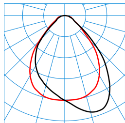
ArimoFit G2 Act D2 P-WW 42-8 ETDD8 01/01 (ACTDSU) TX377596 DIN 5040: A50 UTE: 1,00 C CEN Flux Code: 66 90 97 100 100
