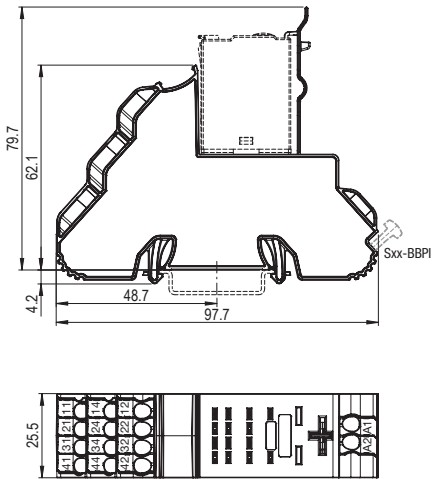
fig. 2. Dimension (mm)
