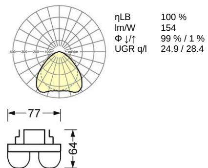
Lighting technology Linear.Lens.Profil-direct wide distribution SDGLB -2 LED 17000 lm 840
