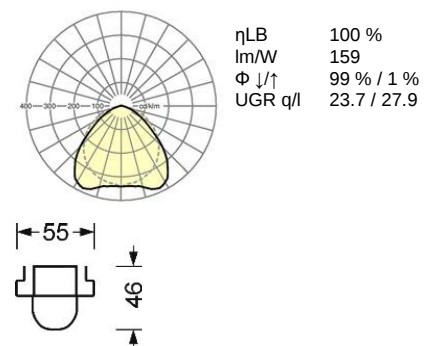
Lighting technology Linear.Lens.Profil-direct wide distribution SDGVLB LED 7500 lm 840
