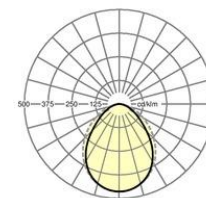
Lighting technology Diffuser, satined-direct distribution RSAGHC-1500 LED 3000 lm 840
