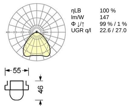
Lighting technology Linear.Lens.Profil-direct wide distribution SDGLB LED 5700 lm 840
