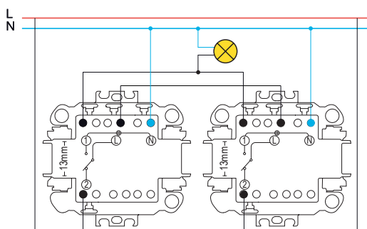
Two 2-way switches with indicator lamps
