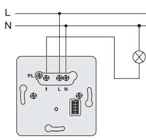
Relay Switch Insert 1-gang
