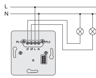
Relay Switch Insert 2-gang
