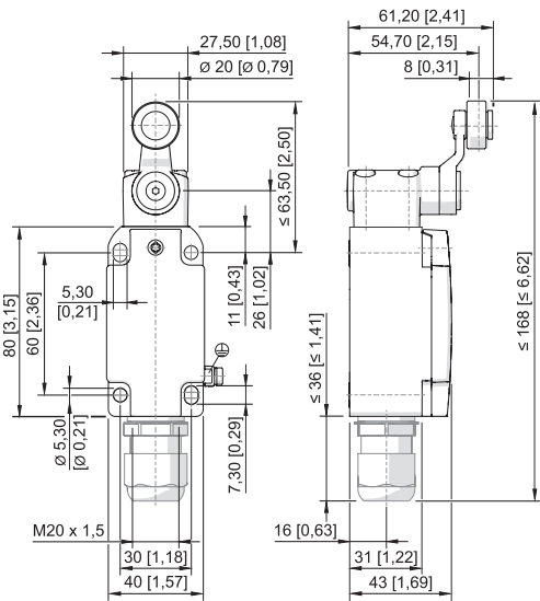
Schwenkhebel 8074/2-1-D-40
