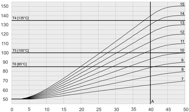
8403/6-5T-5-Ta = 50°C
