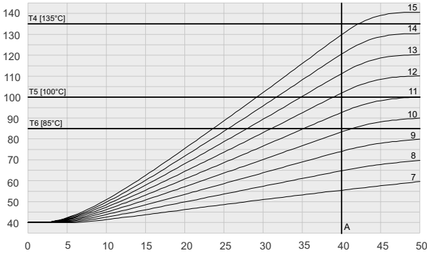
8403/6-5T-5-Ta = 40°C
