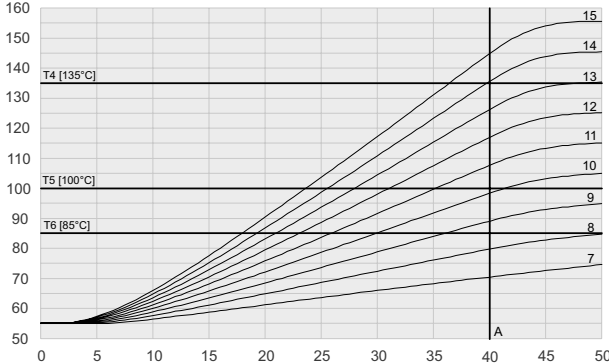
8403/6-5T-5-Ta = 55°C
