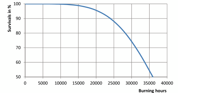
Life Expectancy Diagram - MST SON-T PIA Plus 250W E E40 1SL/12
