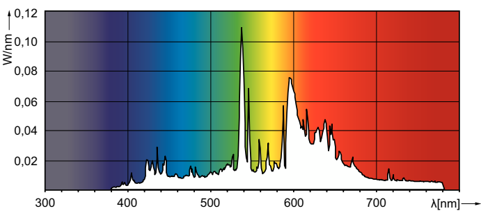
Spectral Power Distribution Colour - CDM-Rm Elite Mini 35W/930 GX10 MR16 10D
