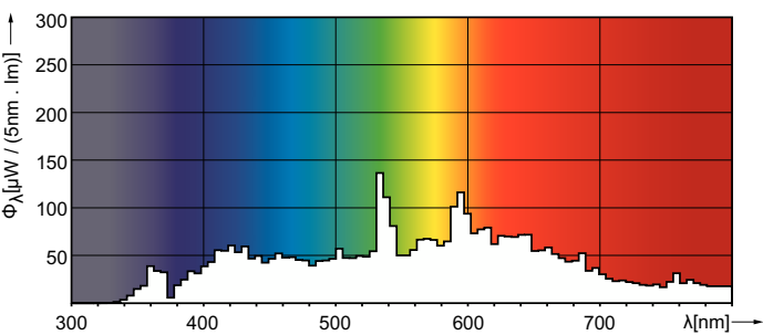
Spectral Power Distribution Colour - MASTERC CDM-R111 70W/942 GX8.5 24D 1CT/6
