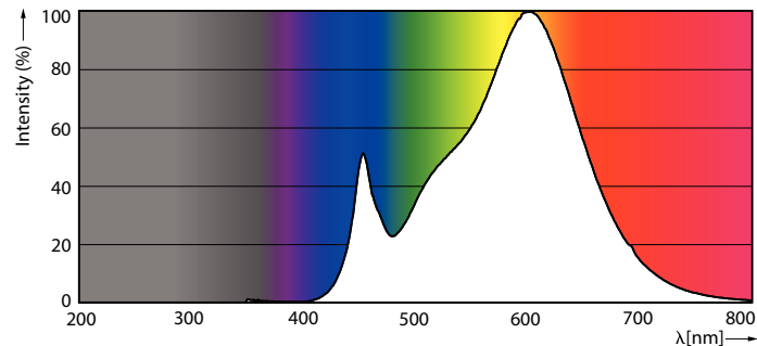
Spectral Power Distribution Colour - TForce Core LED HPL 36W E40 830 FR
