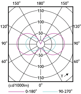
Light Distribution Diagram - CorePro LEDcapsuleLV 1.8-20W G4 827
