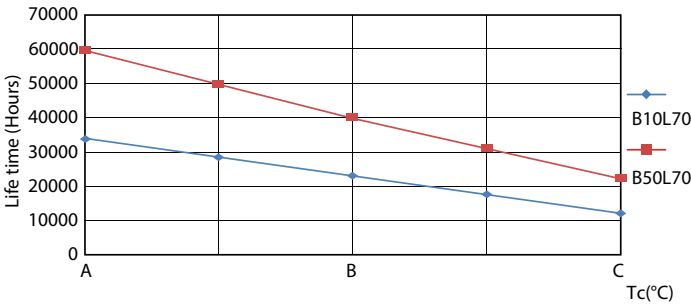
Life Expectancy Diagram - MAS LEDtube HF 1200mm HO 26W 840 T5 OE
