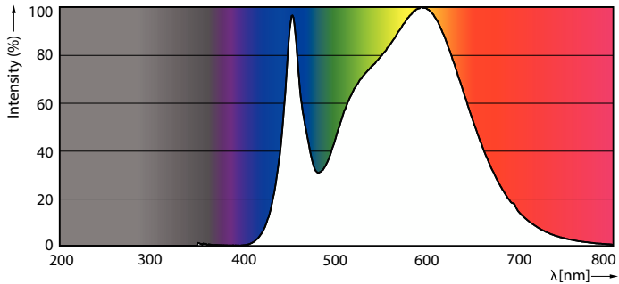
Spectral Power Distribution Colour - TForce Core LED HPL 36W E40 840 FR
