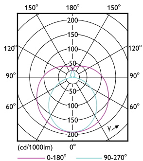
Light Distribution Diagram - MAS LEDtube 600mm HE 8W 840 T5 EU
