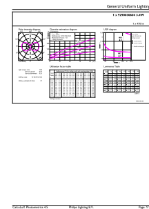
General uniform lighting - MAS VLE LEDLusterD3.4-40W E27 P45 927CLG
