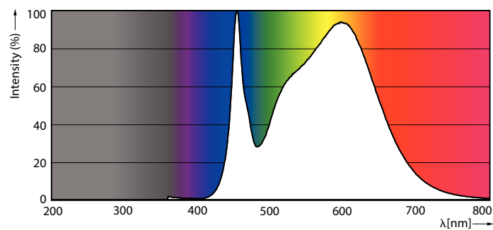
Spectral Power Distribution Colour - TForce LED SOX 28W B22 840 FR
