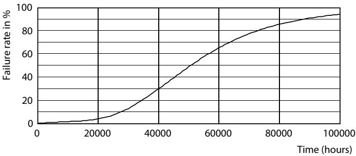
Life Expectancy Diagram - TForce LED SOX 28W B22 840 FR
