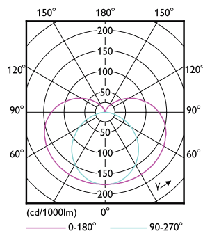
Light Distribution Diagram - TForce LED SOX 28W B22 840 FR
