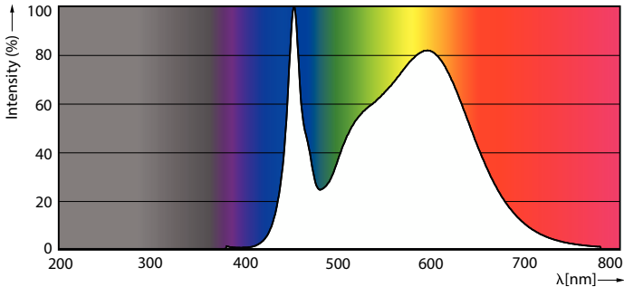
Spectral Power Distribution Colour - MAS LEDtube VLE 1500mm UO 23W 840 T8
