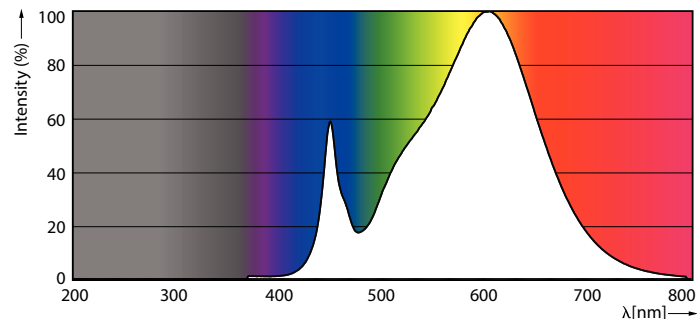
Spectral Power Distribution Colour - MAS LEDtube 1050mm 16W 830 T8
