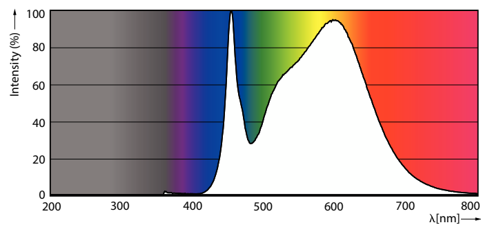
Spectral Power Distribution Colour - TForce LED SOX 18W B22 840 FR
