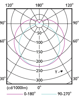
Light Distribution Diagram - MAS LEDtube 1500mm UO 21.7W 865 T8
