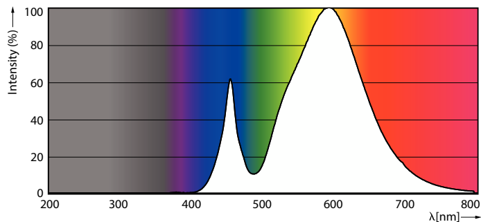
Spectral Power Distribution Colour - TForce Core LED road 40W 730 E40
