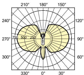
Light Distribution Diagram - MASTERC CDM-T 70W/942 G12 1CT/12
