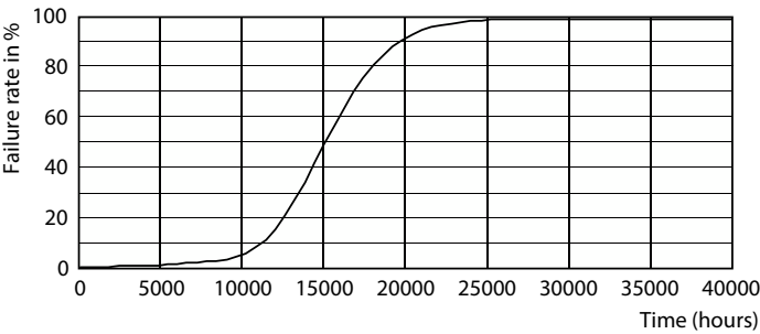
Life Expectancy Diagram - CorePro LEDBulbND 8.5-75W E27 A60 827CLG
