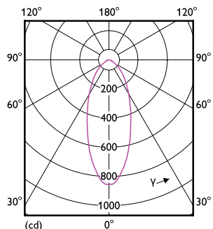
Light Distribution Diagram – MAS LED spot VLE D 6.2-80W GU10 930 36D
