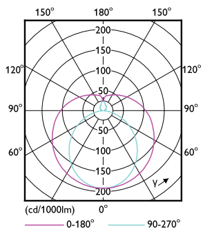
Light Distribution Diagram - MAS LEDtube 600mm HE 8W 830 T5 EU
