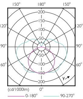
Light Distribution Diagram - CorePro LED linear D 14-120W R7S 118 840
