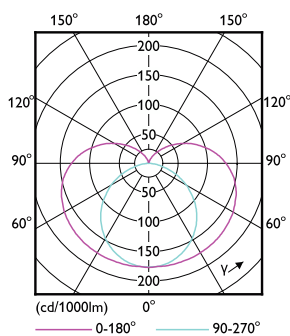
Light Distribution Diagram - TForce LED SOX 36W B22 840 FR
