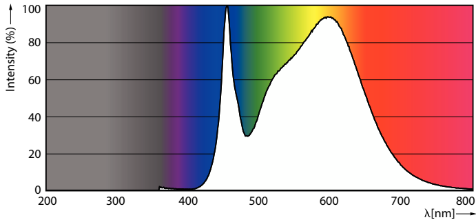
Spectral Power Distribution Colour - TForce LED SOX 36W B22 840 FR
