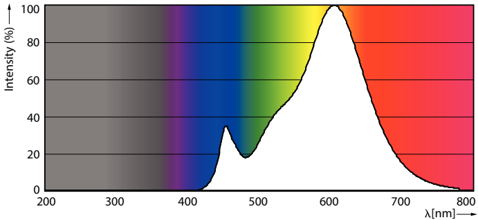
Spectral Power Distribution Colour - CorePro LEDcapsule ND 4.8-60W G9 830
