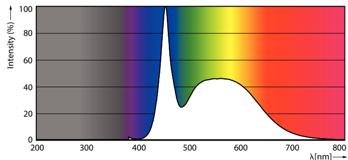
Spectral Power Distribution Colour - MAS LEDtube HF 1200mm HE 16.5W 865 T5
