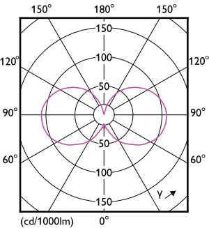
Light Distribution Diagram - MAS LEDLusterDT2.5-25W E27 927 P45CL G
