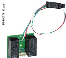
M2C programmable contacts: circuit breaker internal relay with two contacts.
