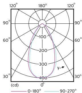
Light Distribution Diagram - MAS LED spot VLE D 4.9-50W GU10 930 60D
