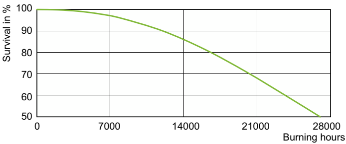
Life Expectancy Diagram - MASTER CityWh CDO-ET Plus 70W/828 E27
