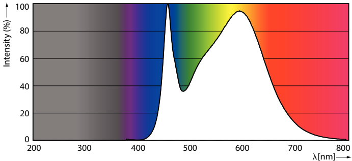
Spectral Power Distribution Colour - CorePro LED linear D 14-120W R7S 118 840
