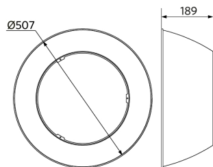
LEDHighbay-E2 Reflector-Rd507
