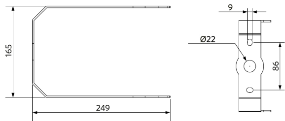
LEDHighbay-E2 Bracket
