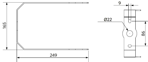
LEDHighbay-E2 Bracket
