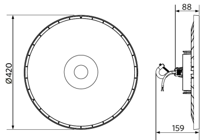
LEDHighbay-E2 Reflector-Rd602
