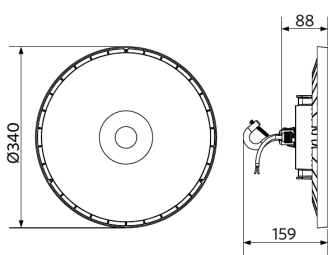
LEDHighbay-E2 Reflector-Rd507
