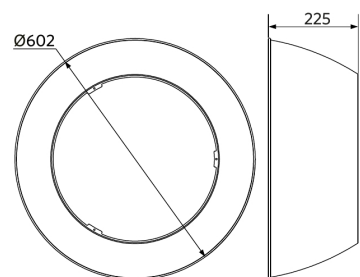
LEDHighbay-E2 Reflector-Rd602
