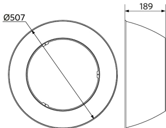
LEDHighbay-E2 Bracket
