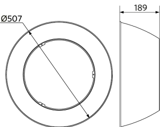
LEDHighbay-E2 Bracket
