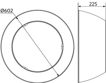
LEDHighbay-E2 Reflector-Rd602
