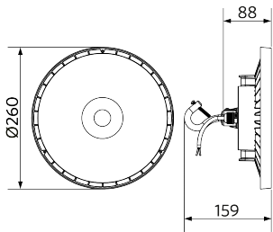
Dimensional_Drawing_HB_E3_70W.png
