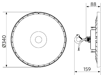
Dimensional_Drawing_HB_E3_110_140W.png
