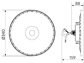
Dimensional_Drawing_HB_E3_110_140W.png
